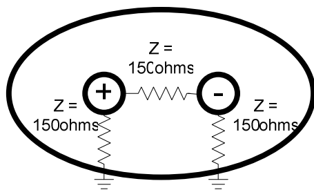
10Cohm Differential Pair Twisted Pair or Twinax
